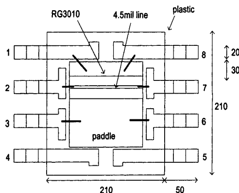
Fig. 1. Classic SSOP8 pin package with 50\Omega through inserted between ports 2 and 7.
