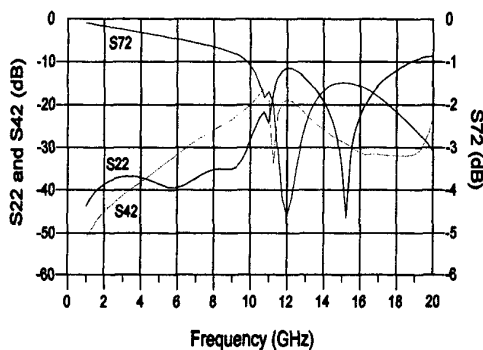
Fig. 6. HFSS simulation of proposed modified SSOP8 ECPWFG package, showing improved performance to 10 GHz. The lower frequency resonances have been minimized by redesign of the lead frame transitions.
